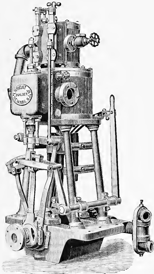
WRIGHT'S LAUNCH ENGINE.—6½, 13 x 8.
